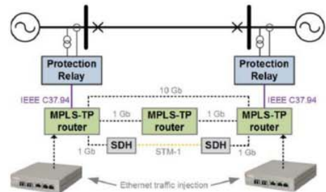
Fig. 5. Ethernet load injection
