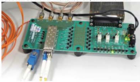
Fig. 6. Reproducible fiber cut hardware
