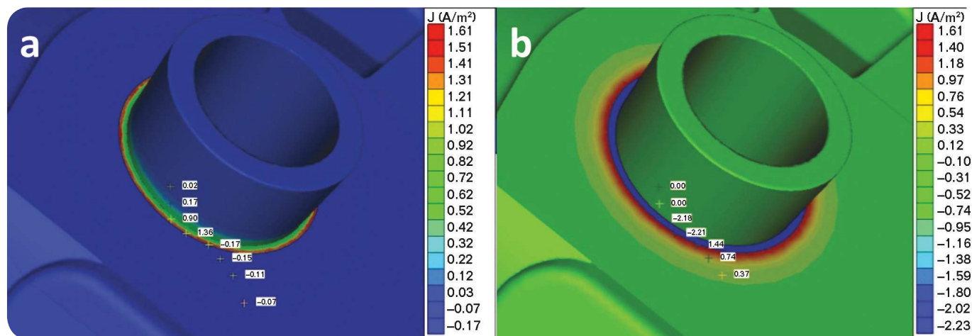
FIGURE 2 Corrosion currents for the wing lug assembly: (a) anodized Al, Cd-plated CuBe, and steel; (b) anodized Al, bare CuBe, and steel.
