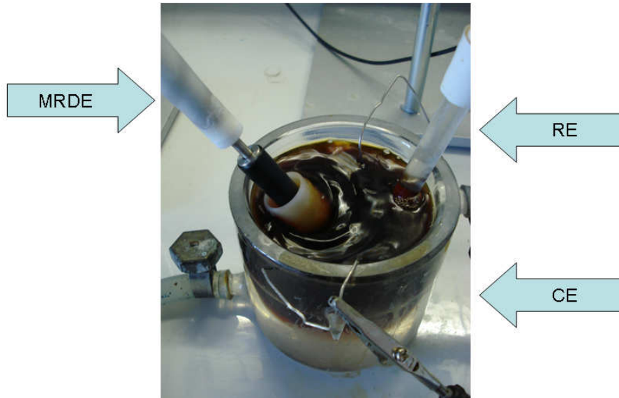
Figure 2 – MRDE laboratory set-up
