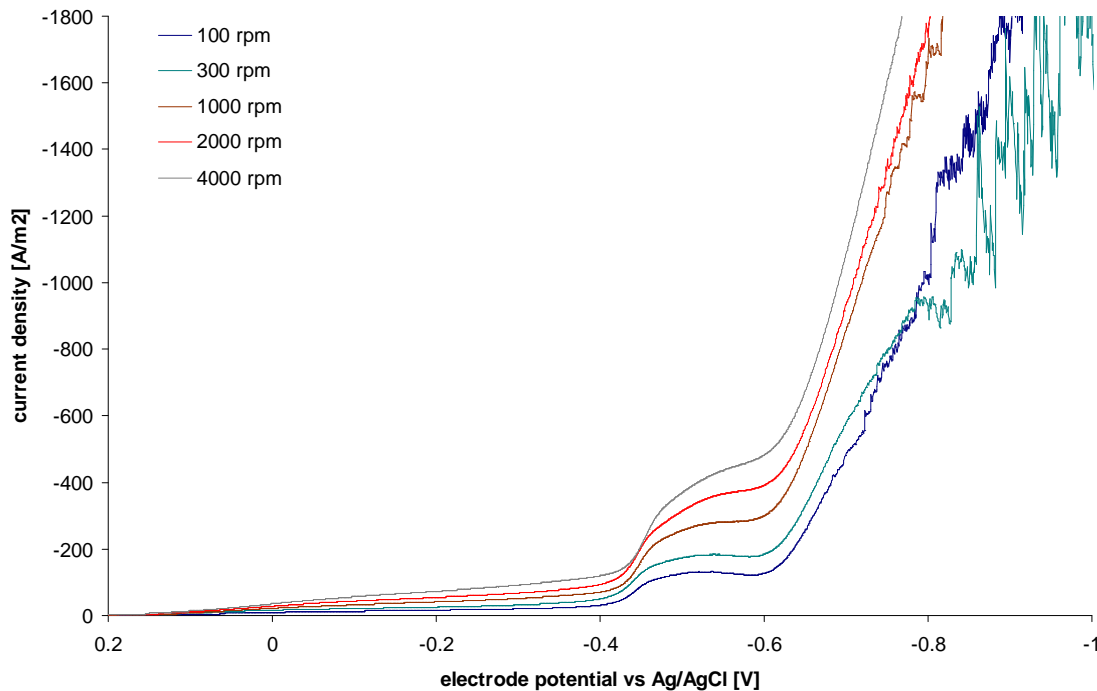
Figure 4 – Example of a platinum electrolyte polarization curve
