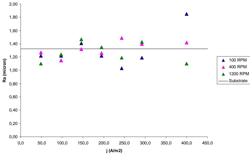
Figure 8 – Roughness as function of current density
