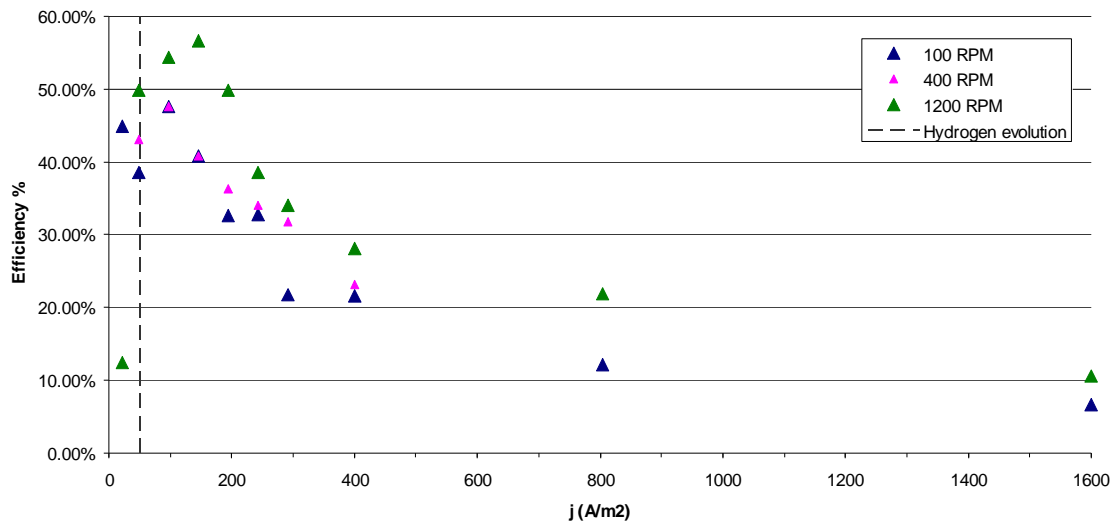
Figure 6 – Efficiency as a function of current density for 3 different rotation speeds
