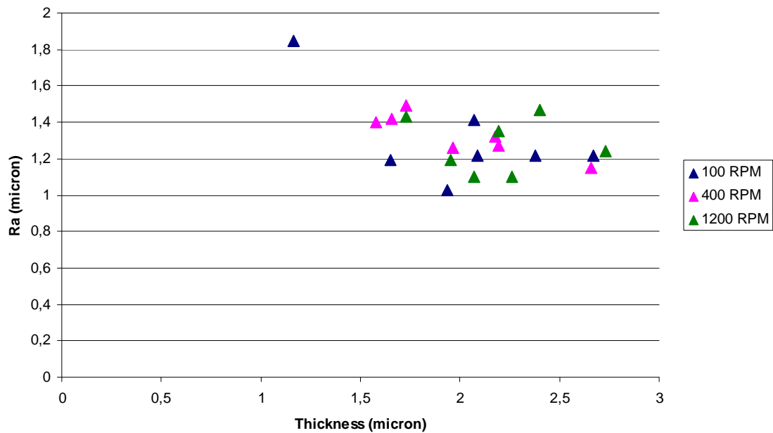
Figure 9 – Roughness as function of layer thickness values
