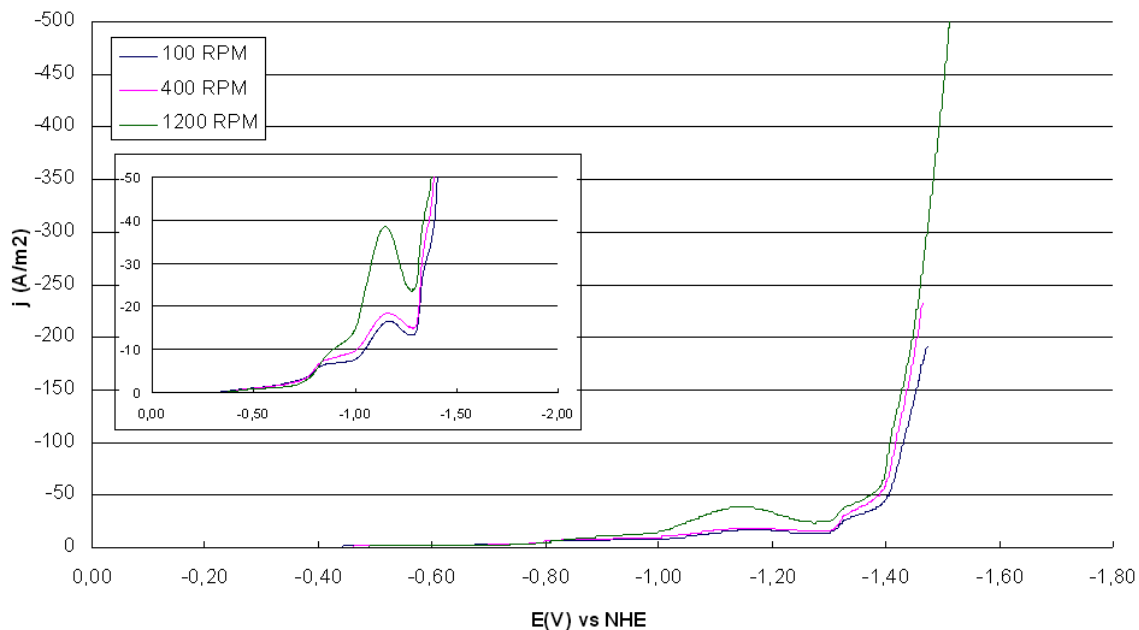
Figure 5 – Polarization curves for 3 different rotation speeds
