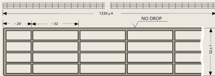
Cross-section of PLEXIGLAS® Heatstop Opal S5P 32 (dimensions in mm)
